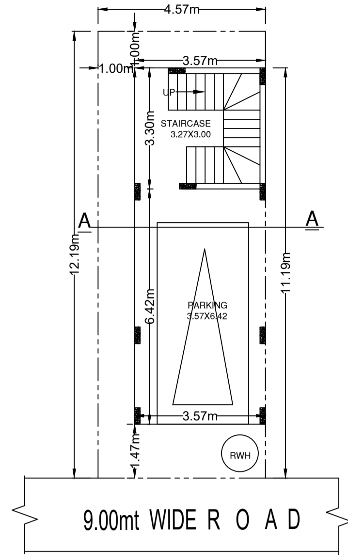
PROPOSED STILT FLOOR PLAN
