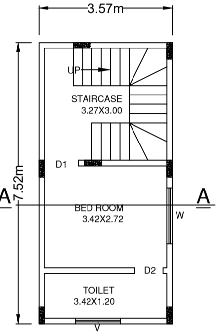
PROPOSED SECOND FLOOR PLAN
